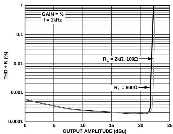
Figure 33. THD + N vs. Output Amplitude, G = \frac{1}{2}
