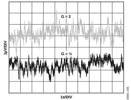
Figure 38. 0.1 Hz to 10 Hz Voltage Noise, RTO
