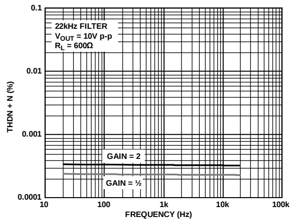
Figure 31. THD + N vs. Frequency, Filter = 22 kHz
