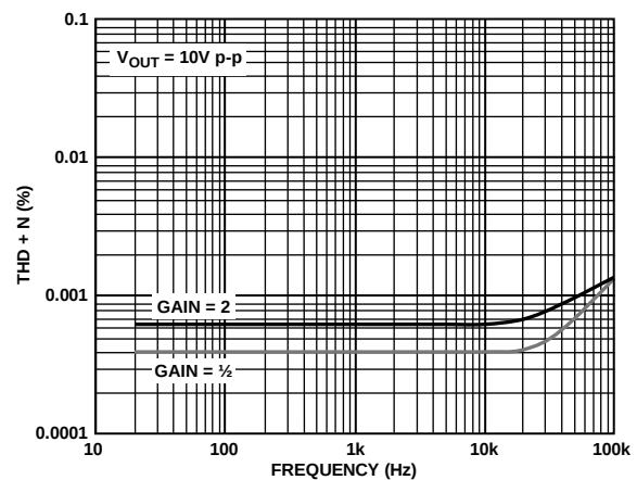
Figure 32. THD + N vs. Frequency, Filter = 120 kHz
